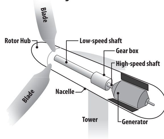
Wind Turbine Diagram
